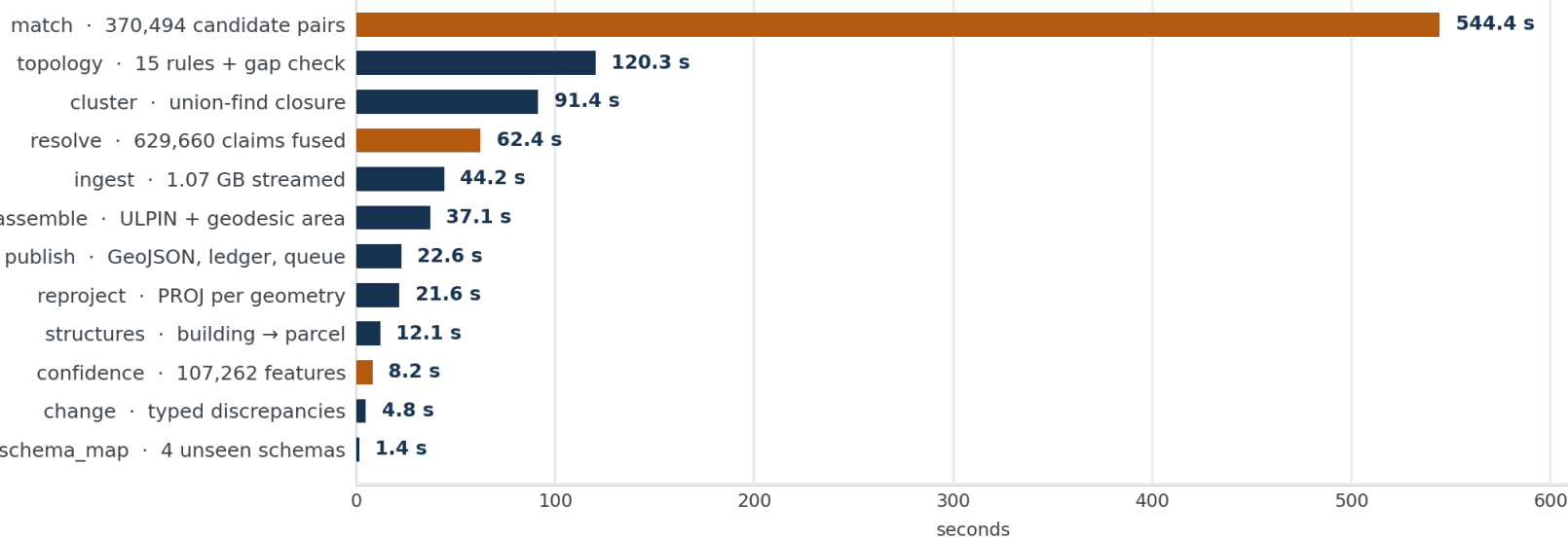
Wall-clock by pipeline stage — 1,065 s (17 min 45 s) end to end on 2 vCPU / 7 GB
